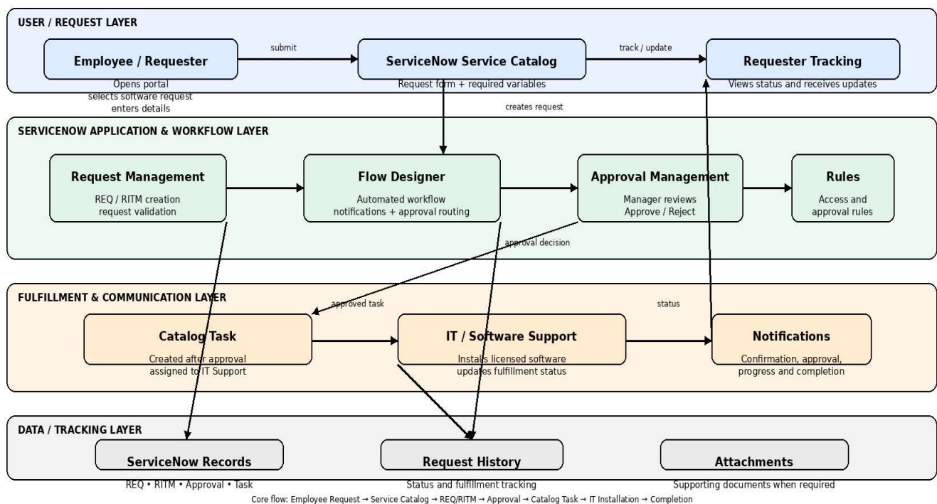
Figure 1: Solution architecture and data flow for the ServiceNow licensed software request process
